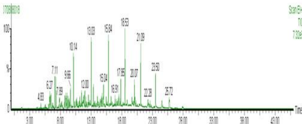
Fig. 1.7 (a) Chromatogram of fire debris sample
