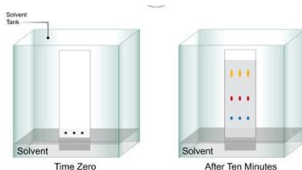
Figure 3: The solution is applied near one end of a plate coated with silica or alumina. The plate is then immersed in a solvent, which rises up the plate by capillary action. In most situations, visualization is by way of a spray reagent, generally a modified Griess reagent which will identify nitro groups present within the explosive molecule. The technique is still widely used though it has been largely superseded by instrumental techniques.
