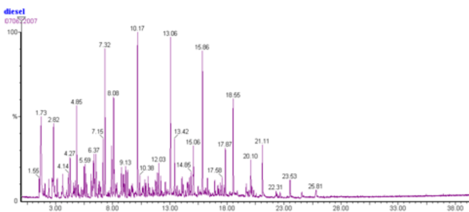
Fig. 1.7 (b) Chromatogram of diesel standard
