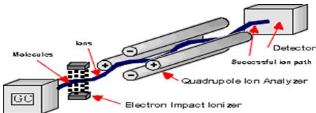
Fig 1.5: Schematic representation of a Mass Spectrometer
